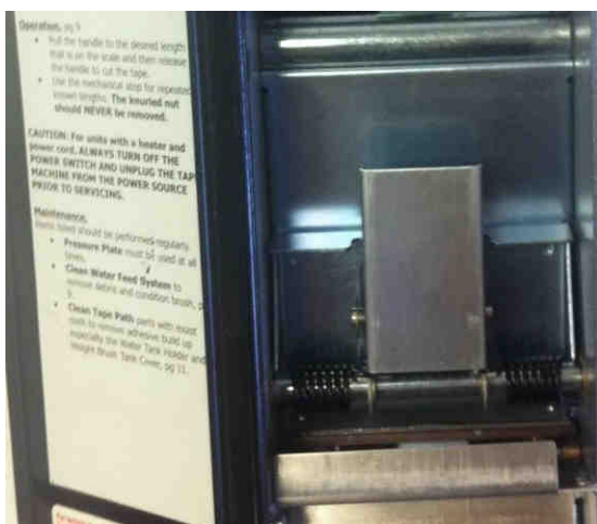
Fig 13 Pinch Roller, Serial Numbers 601082 and Above
