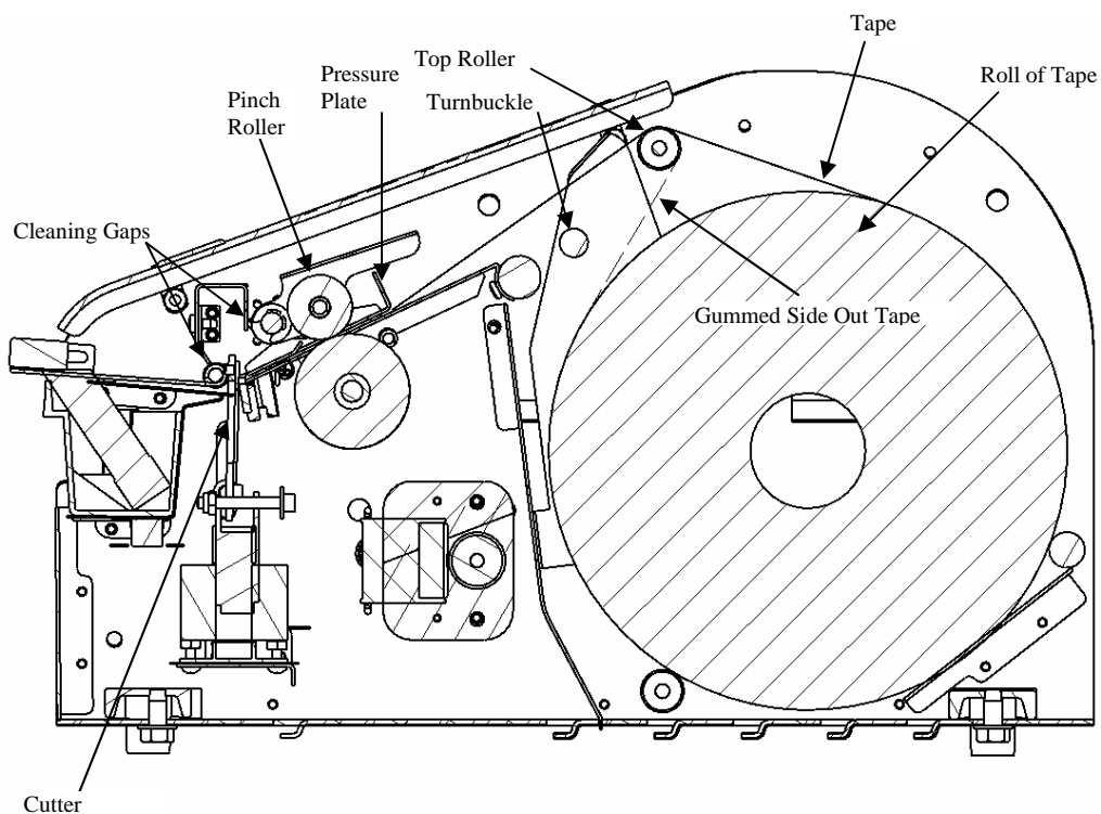
Figure 3 – Tape Routing
